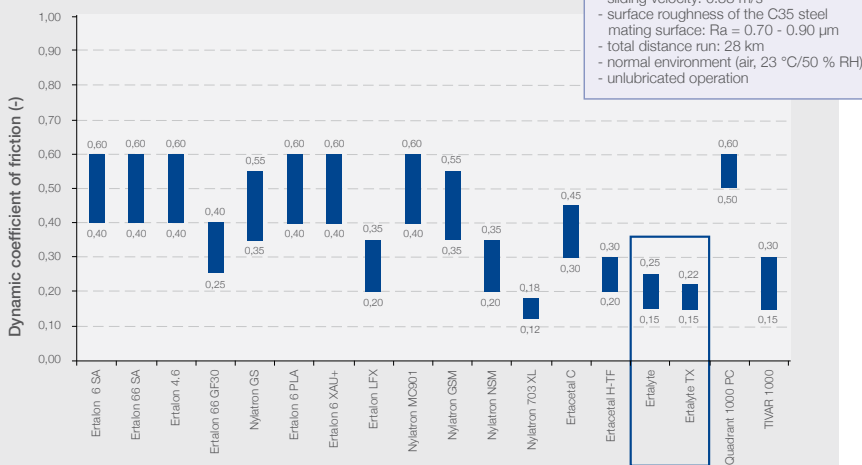
Fig. 1 Dynamic coefficient of friction (measured on a "plastics pin on rotating steel disk" - tribo system)
